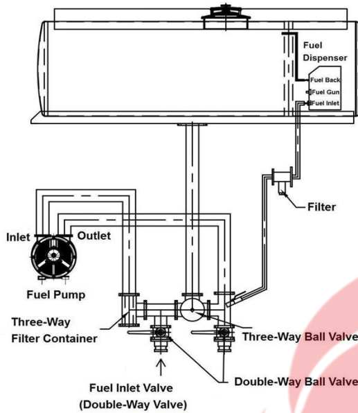
Fuel Truck Pipeline System
